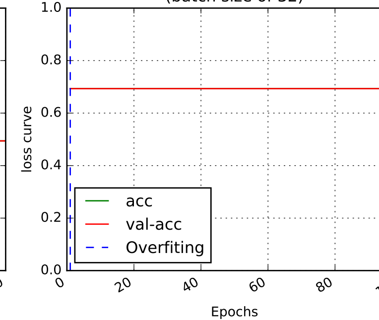
(b) SqueezeNet loss curve (batch size of 32)
