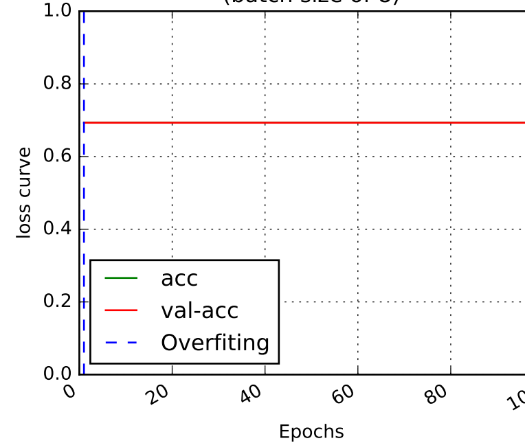
(b) SqueezeNet loss curve (batch size of 8)
