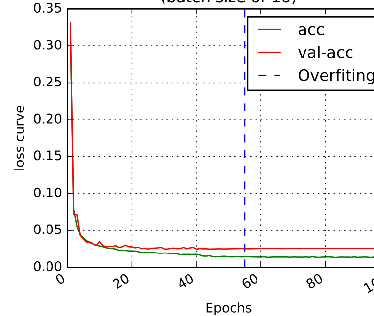
(b) ResNet loss curve (batch size of 16)
