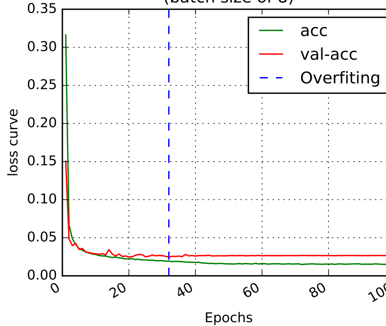
(b) ResNet loss curve (batch size of 8)
