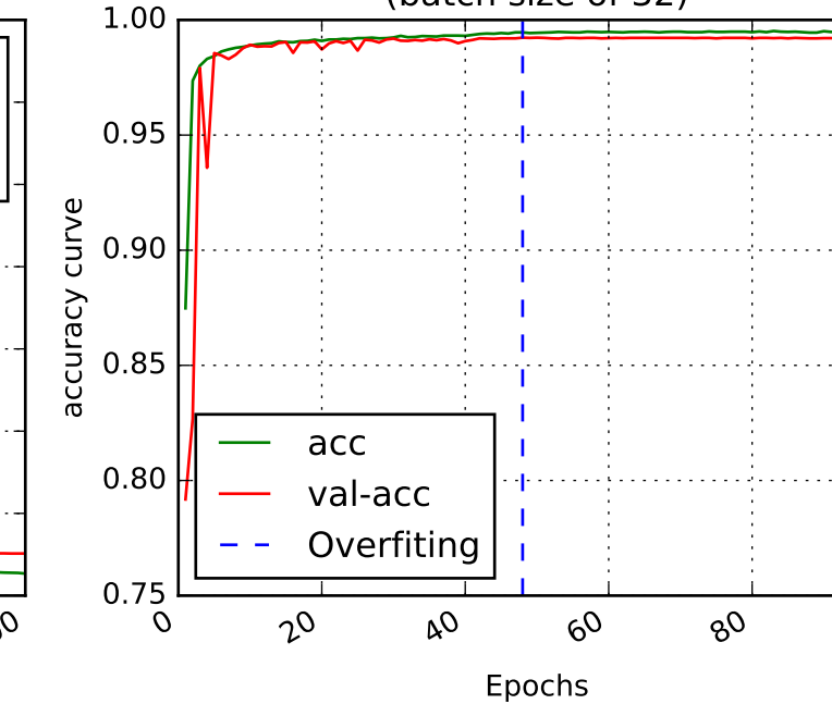
(a) ResNet accuracy curve (batch size of 32)
