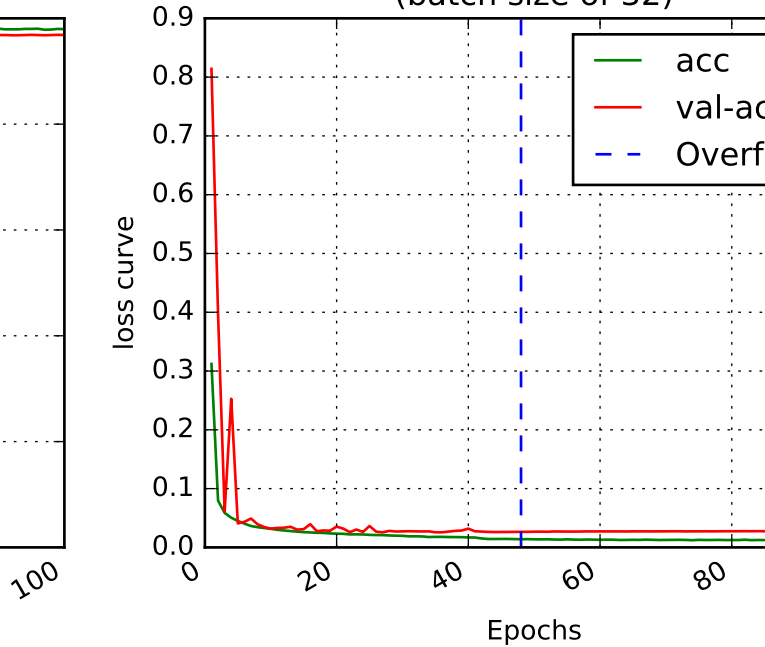
(b) ResNet loss curve (batch size of 32)
