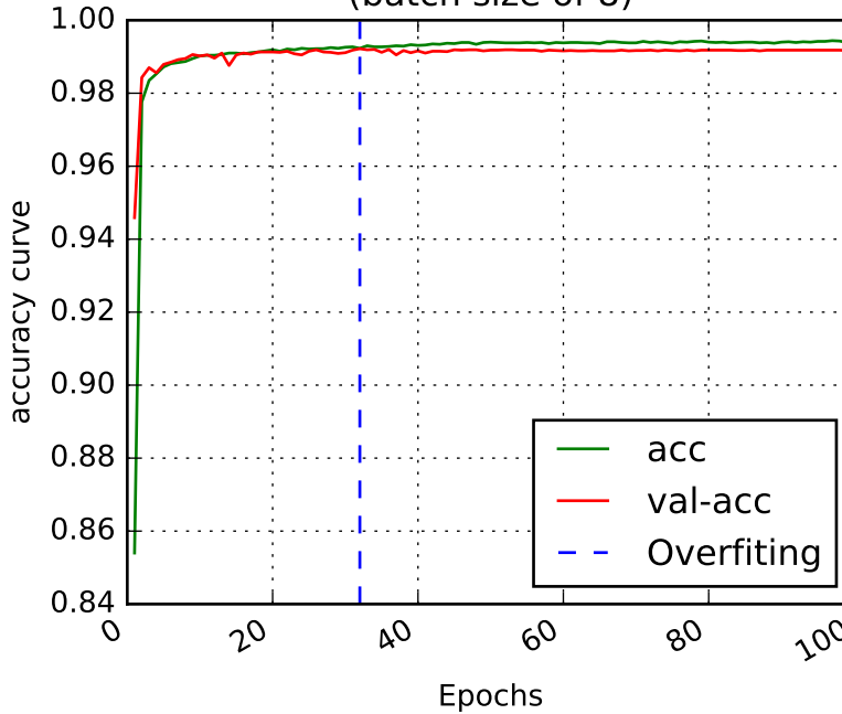
(a) ResNet accuracy curve (batch size of 8)
