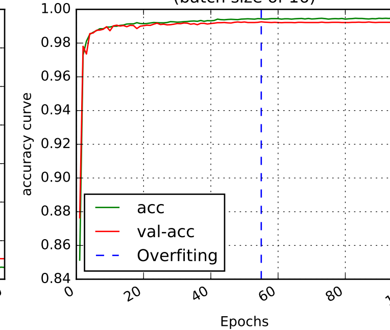
(a) ResNet accuracy curve (batch size of 16)
