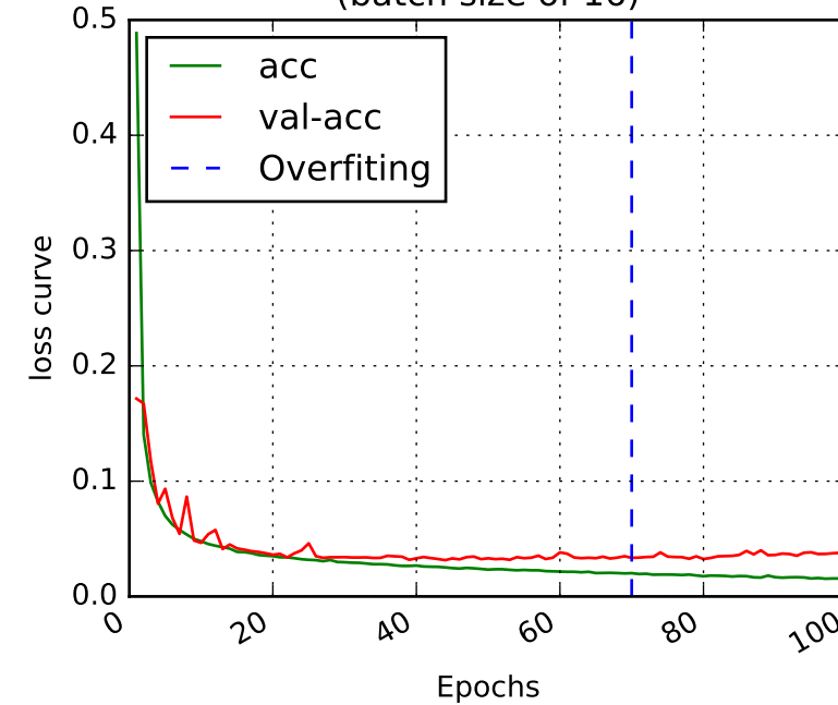
(b) DenseNet loss curve (batch size of 16)
