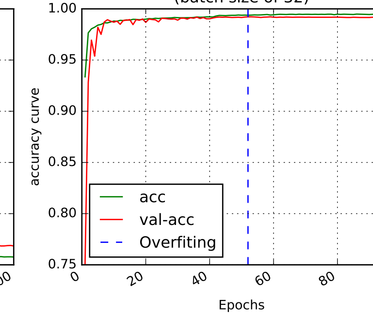
(a) DenseNet accuracy curve (batch size of 32)
