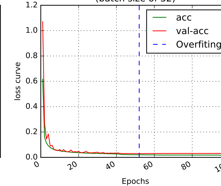
(b) DenseNet loss curve (batch size of 32)
