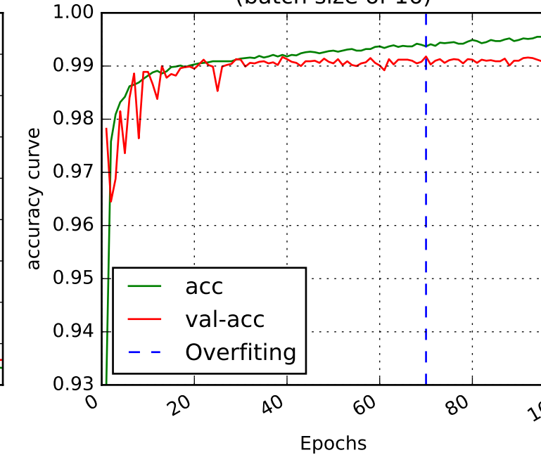
(a) DenseNet accuracy curve (batch size of 16)
