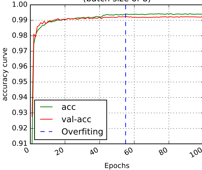
(a) DenseNet accuracy curve (batch size of 8)
