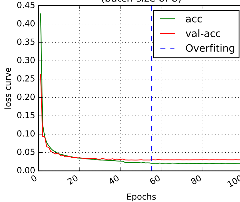
(b) DenseNet loss curve (batch size of 8)
