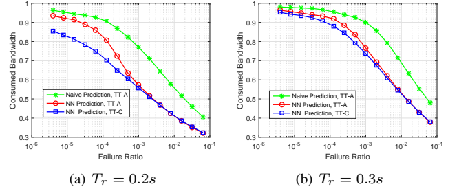
Fig. 9. The comparison of TT-A and TT-C.
