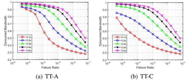
Fig. 8. The consumed bandwidth v.s. failure ratio
